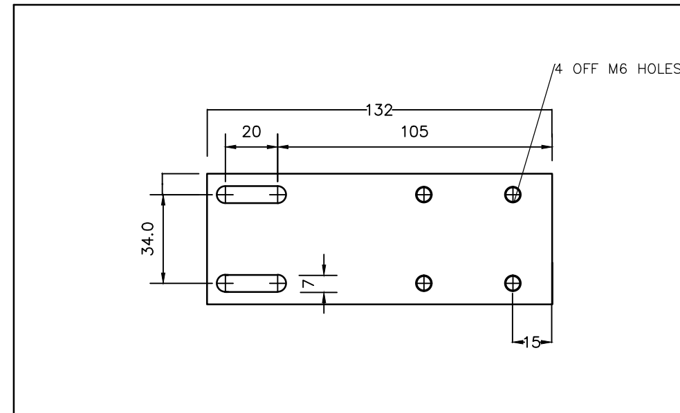
ED-2768/2 Flat Plate Slotted (1)
