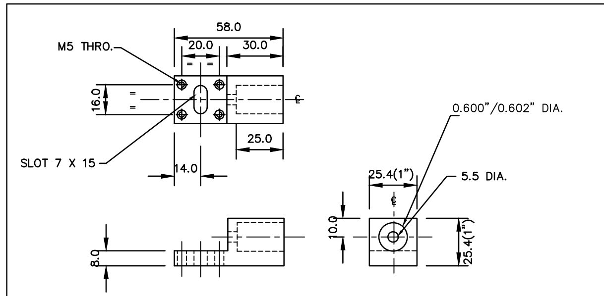
ED-2768/4 Flat Plate (1)
