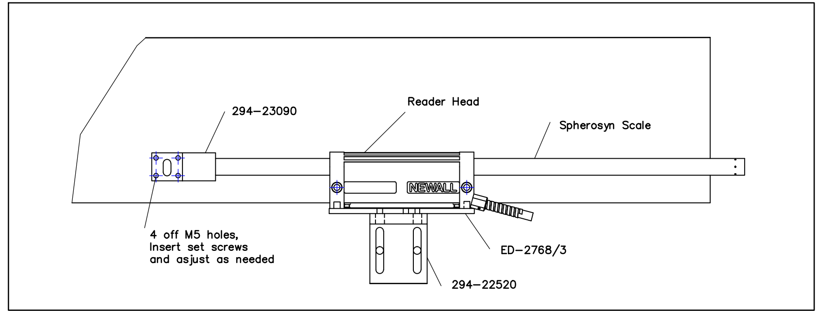
Cross Slide (X-axis)
