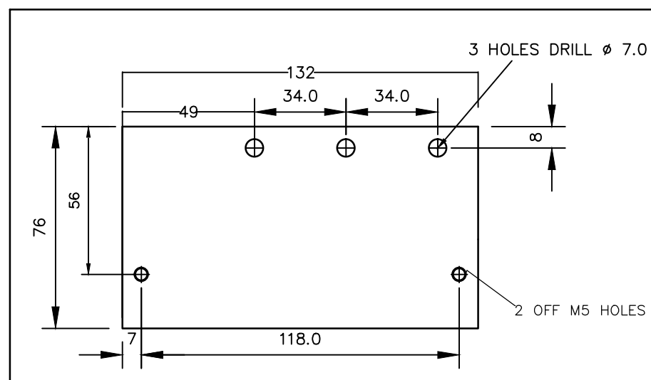
ED-2768/4 Flat Plate (1)
