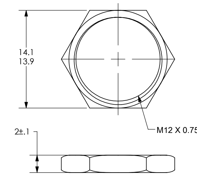
DETAIL "A" MOUNTING NUT BLACK FINISH SCALE 3:1
