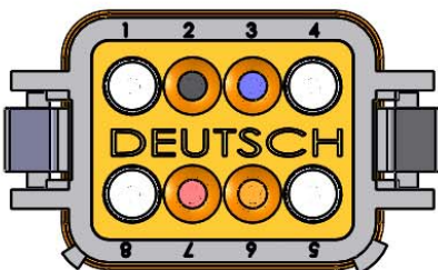
0857-9 CAN-Bus
