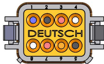
0857-8 Delay on Break with Auxiliary
