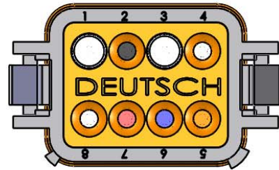
0857-6 Low Voltage Disconnect with Auxiliary
