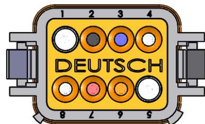
0857-10 CAN-Bus with Auxiliary
