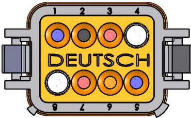
0857-3 Over Current
