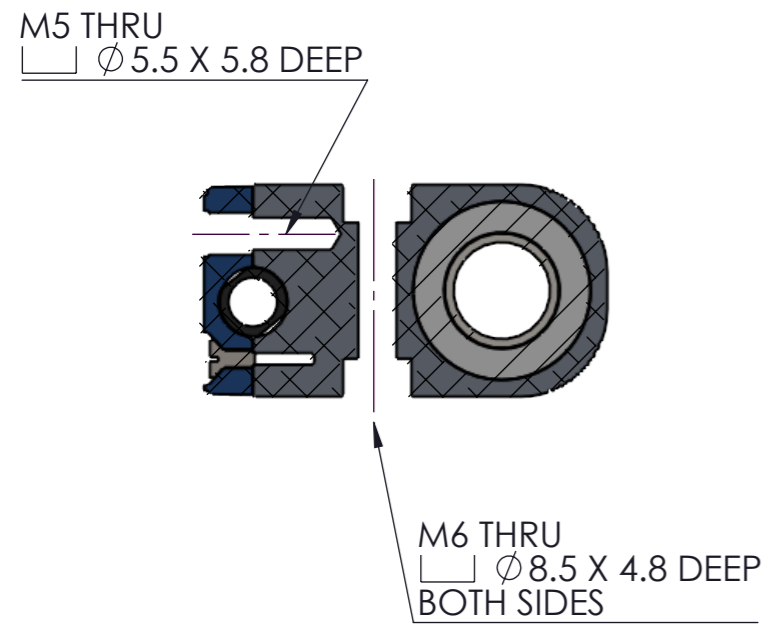
MOUNTING HOLE DETAILS SECTION A-A SCALE 1 : 1
