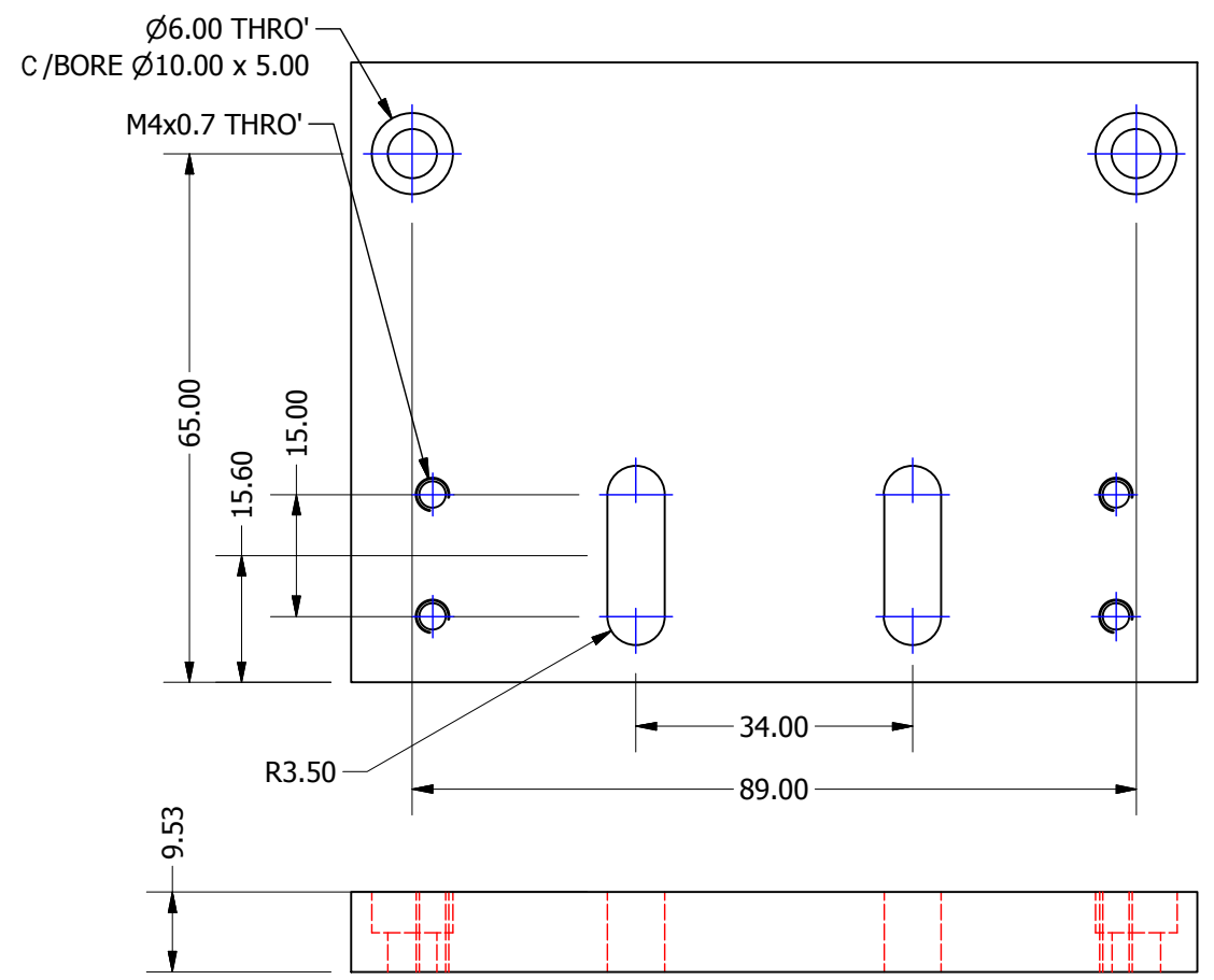
(QTY 2) 295-00990 PLATE BRACKET
