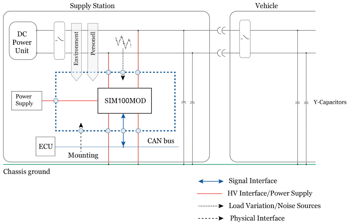
Figure 3: The boundary diagram of SIM100 as SEoC in EV implementations
