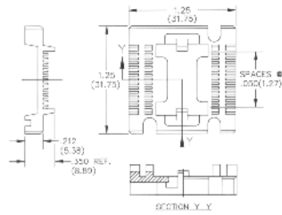
Drawing of 28-lead carrier (others available upon request)
