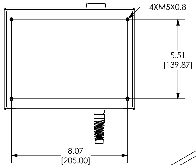
VIEW A-A SCALE 1 : 4
