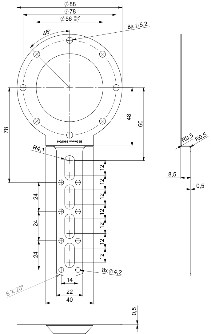
Tether Arm for DSU9
