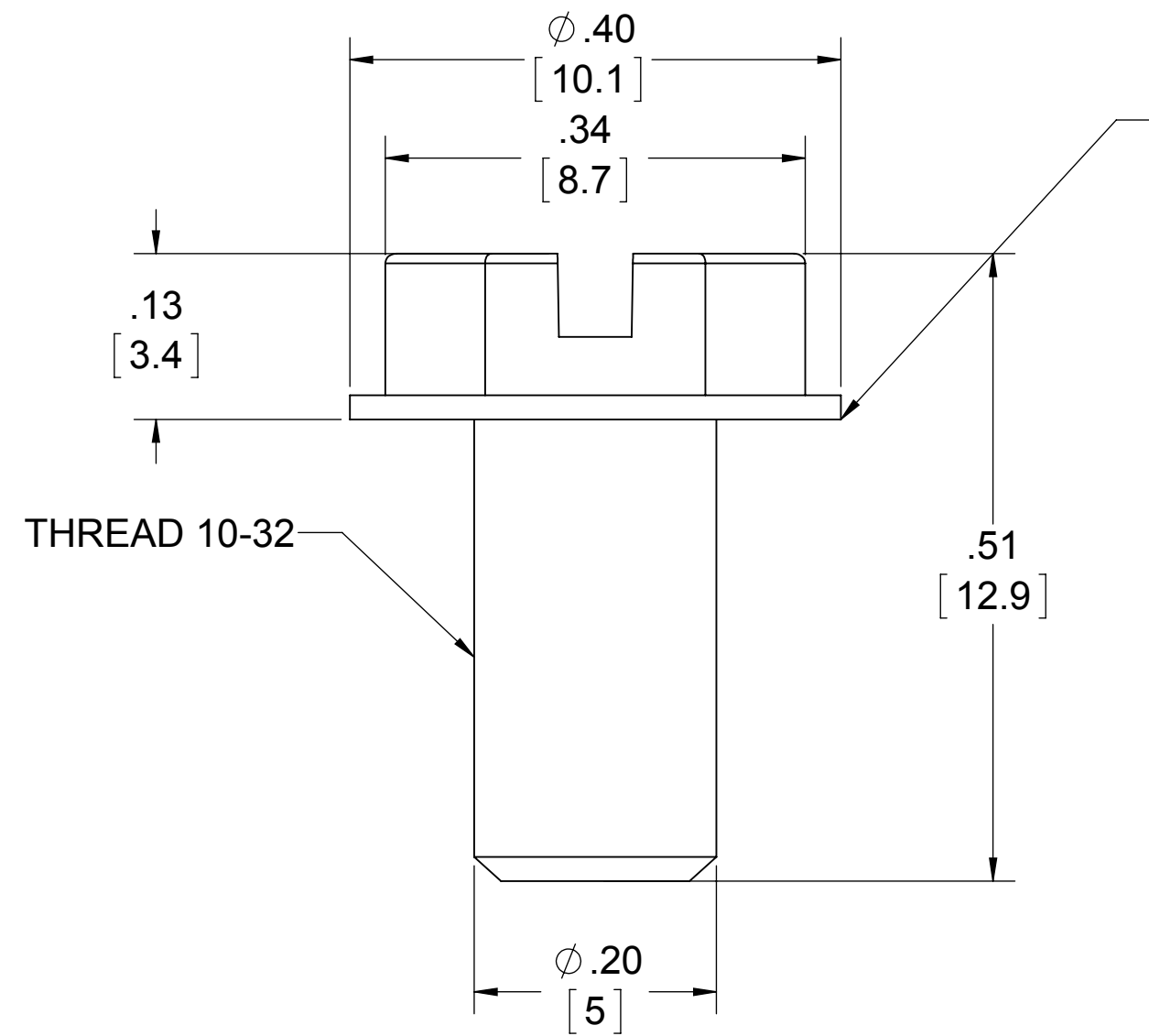
GROUND SCREW (1 PLACE) (PART REF 107620)
