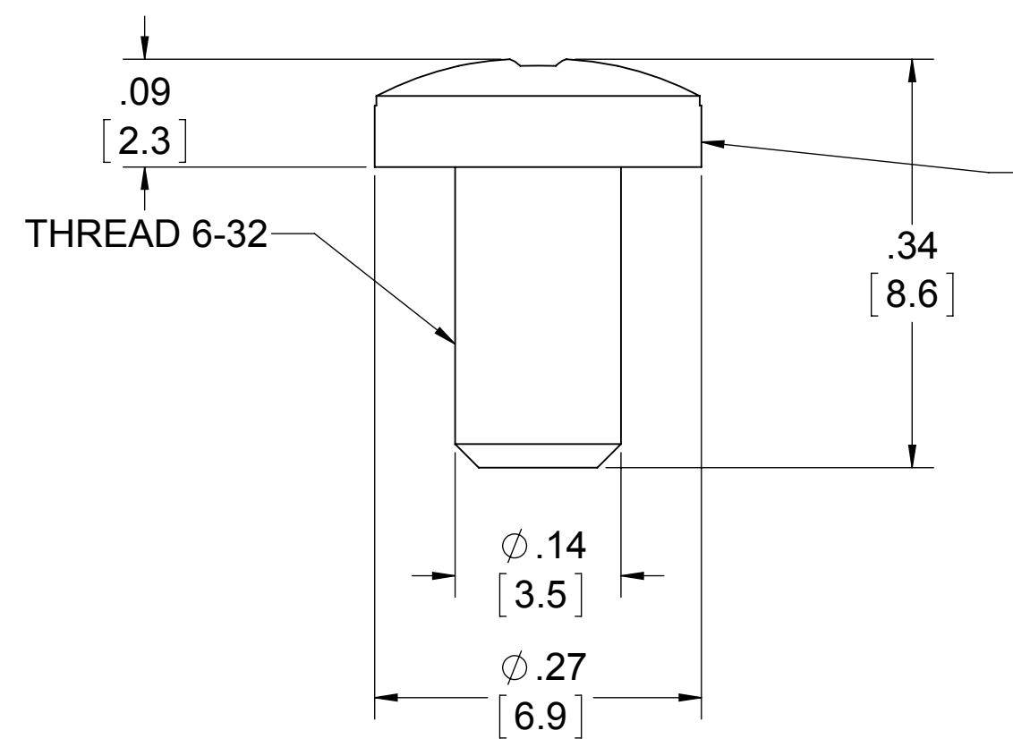
MOUNTING SCREW (2 PLACES) (PART REF. 107621)
