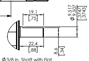
Ø3/8 in. Shaft with Flat
