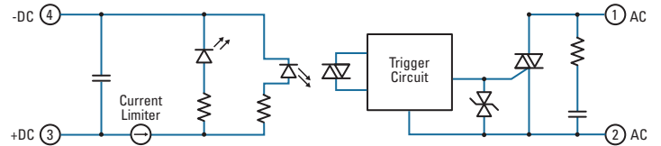
Diagram 6: DC60 Series, DC Control
