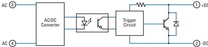
Diagram 7: 1-DC, 1-DCL, D1D, D06D Series
