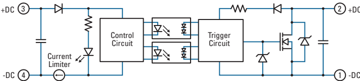
Diagram 9: PowerPlus DC Series
