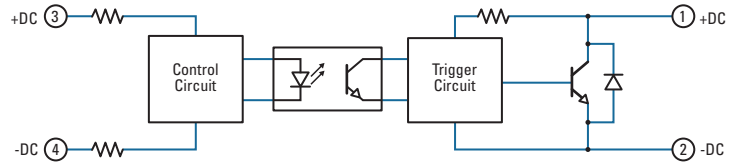
Diagram 8: SSC Series
