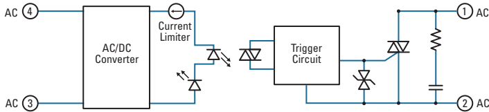
Diagram 5: DC60 Series AC Control
