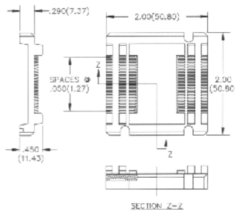
Drawing of 40-lead carrier (others available upon request)
